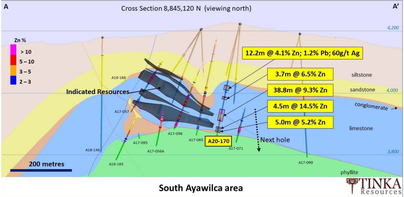
Figure 2. Cross section of drill hole A20-170
