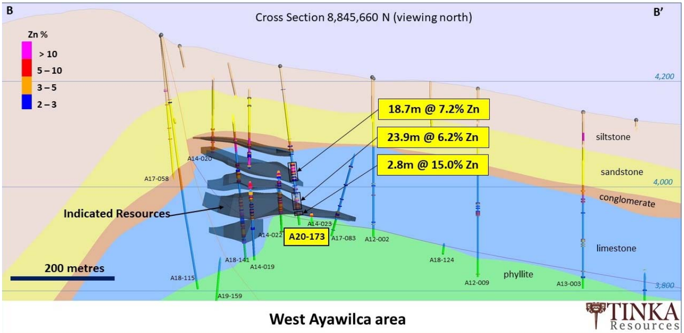
Figure 3. Cross section of drill hole A20-173
